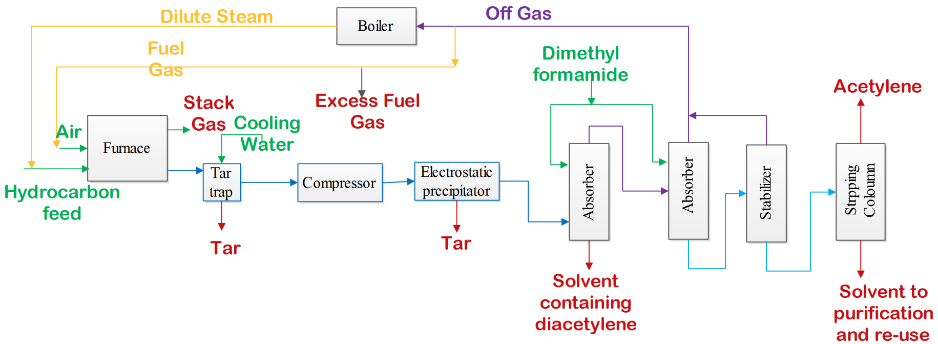
Figure: Manufacture of Acetylene by Wulff Process
